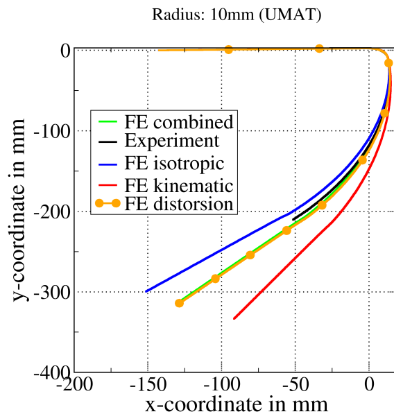
Figure 8: Draw bending (Experiments IUL)
