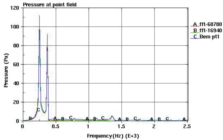
Figure 7: Comparison of Kirchoff method to FEM of LS-DYNA®
